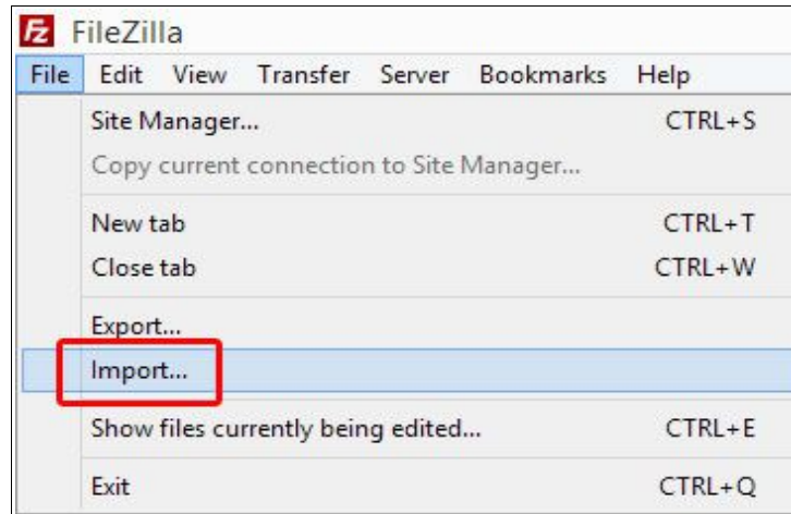
Figure 3.1 Import file
