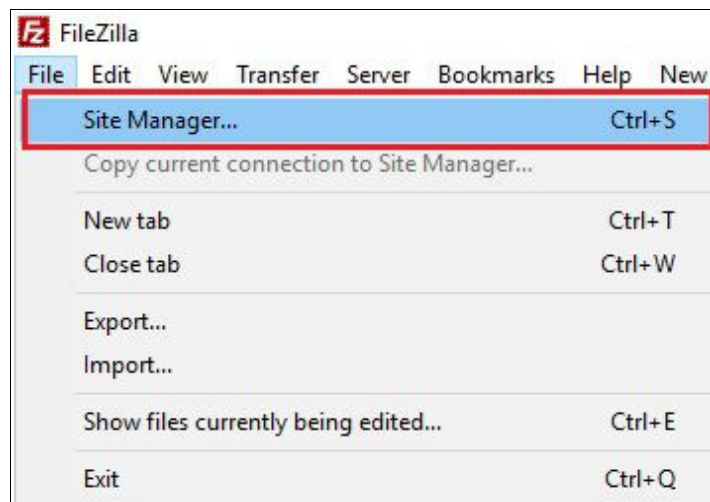
Figure 4.1 Site Manager
